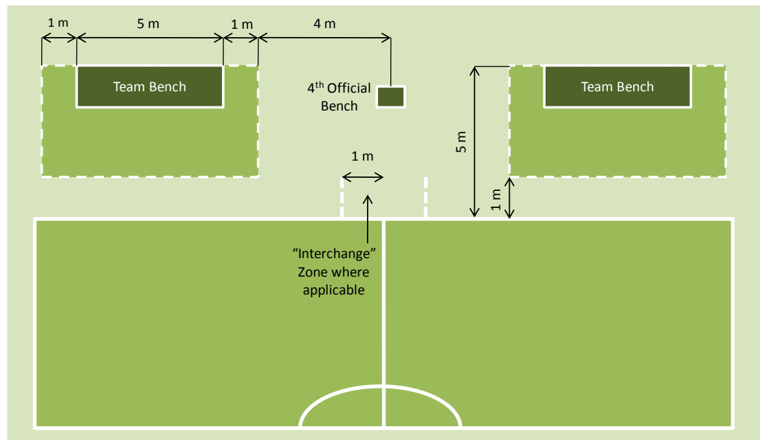
Diagram 5 - Technical Area line marking and dimensions
